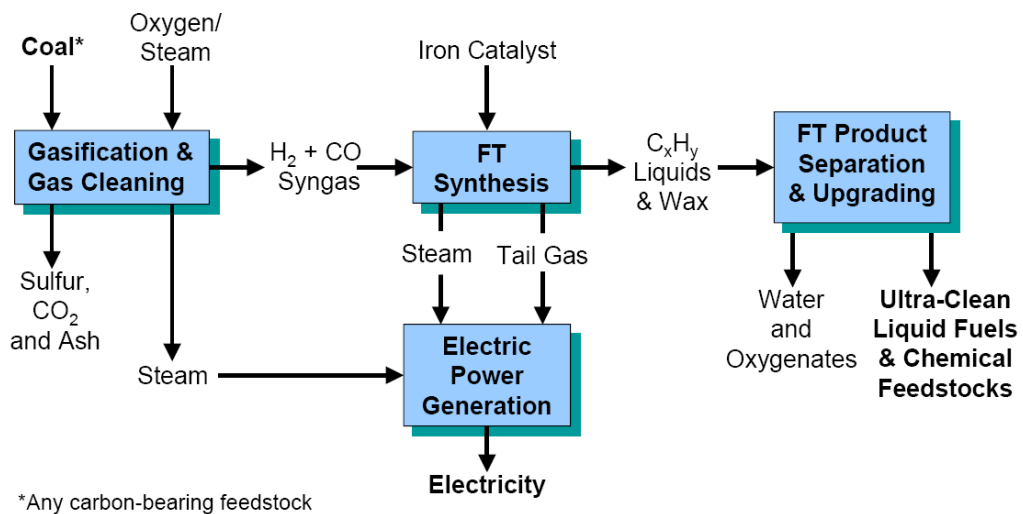
Figure 4. Process Flow Diagram for CTL facility.
